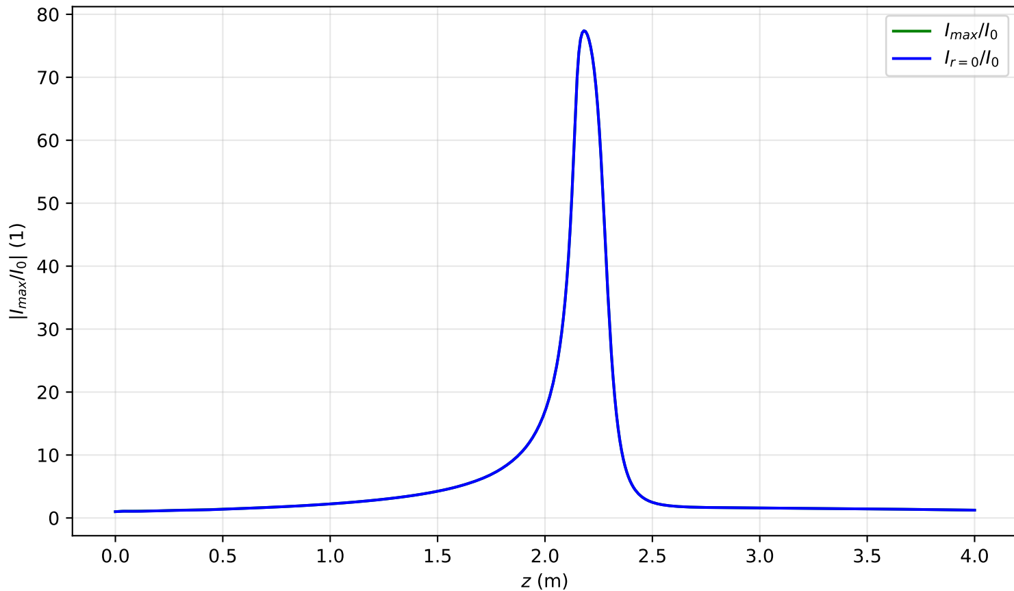
I_{max}(x=0, y=0, z)/I_0 , Pin=1.3Pcr, noisy input, artificial time
